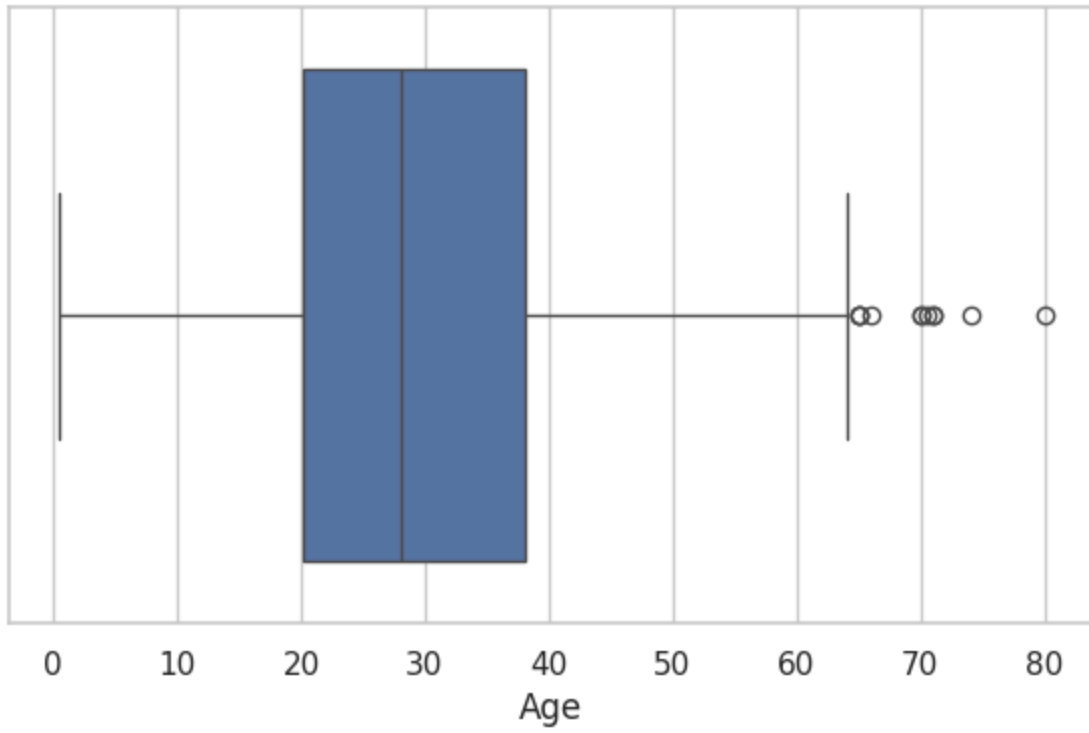
Age Boxplot
